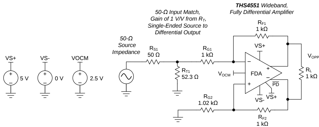
Figure 74. DC-Coupled Gain of 1 with R_F = 1 \text{ k}\Omega and Single-to-Differential Matched Input 50-Ω Impedance
