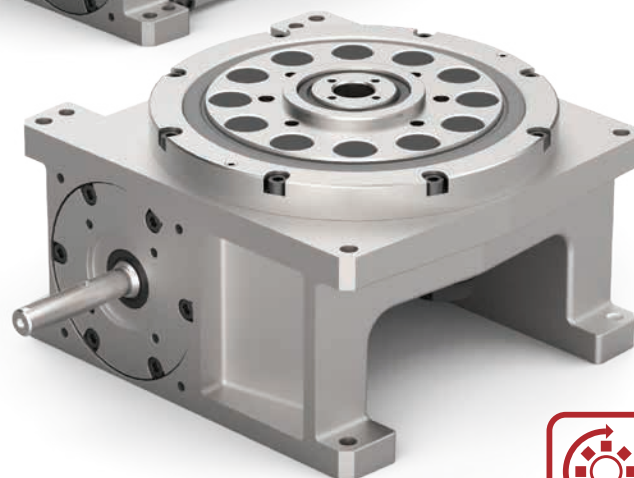
BCD50 shown with motor and gearbox.
