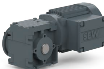
SEW / WAF Gearbox and Motor without Brake.
