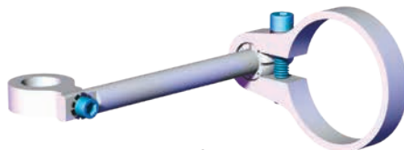
18mm Swivel Proximity Sensor Mount
