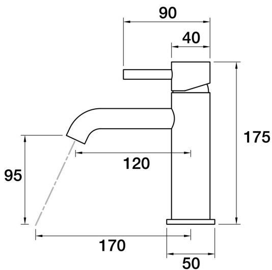
Lugano Hob Basin Mixer A22.011.2.34 - Matt Black
