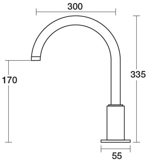
Portsea Sink Hob Swivel Outlet X/Large D29.032.2.01 - Chrome
