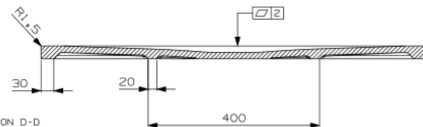
SECTION D-D SCALE 0.143:1.0
