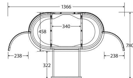
TOP VIEW: DRAWER & DOORS OPEN
