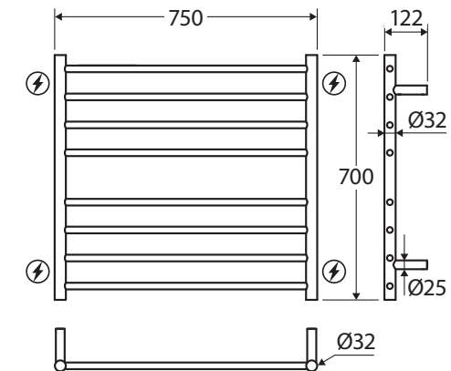
⚡ Wiring Positions
