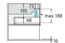
SIDE VIEW: DRAWER STORAGE
