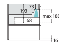
SIDE VIEW: DRAWER STORAGE
