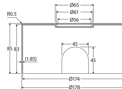
Cover Plate
