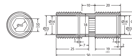
Water Inlet G \frac{1}{2} Thread
