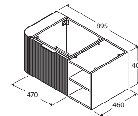
Cabinet with Undermount Basins & select Select Semi inset basins
