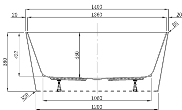
Cross Section F-F
