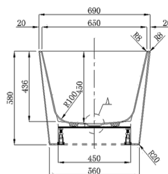
Cross Section G-G
