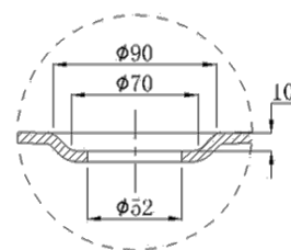
Enlarged Drawing A
