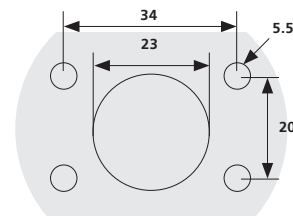
Mounting Specifications (mm)
