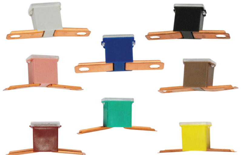
PAL – Male Terminations (13/16" Bent) Auto Link Fuses
