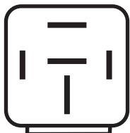
2 x 1/4" & 3 x 3/8" Terminals
