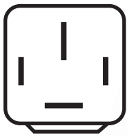
2 x 1/4" & 2 x 3/8" Terminals
