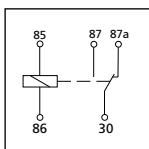
5 x 1/4" Terminals
