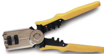
Heavy-Duty Wire Stripper 669967 This heavy-duty wire stripper has a built in crimper/cutter. Good for 22 - 10 AWG insulated and non-insulated terminals.
