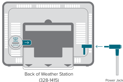
Power Jack
