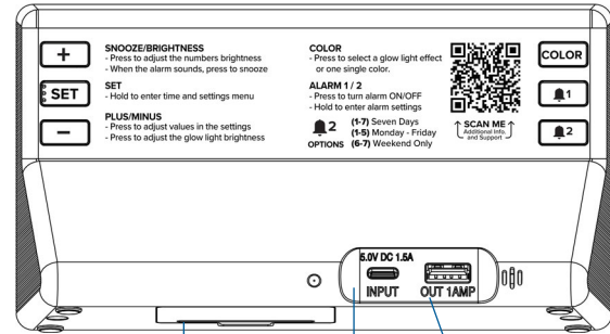
- AAA + Battery + AAA - Compartment for optional 2-AAA batteries. USB-C Port to Power the Clock USB-A Charging Port for your external device. Charging cord not included.
