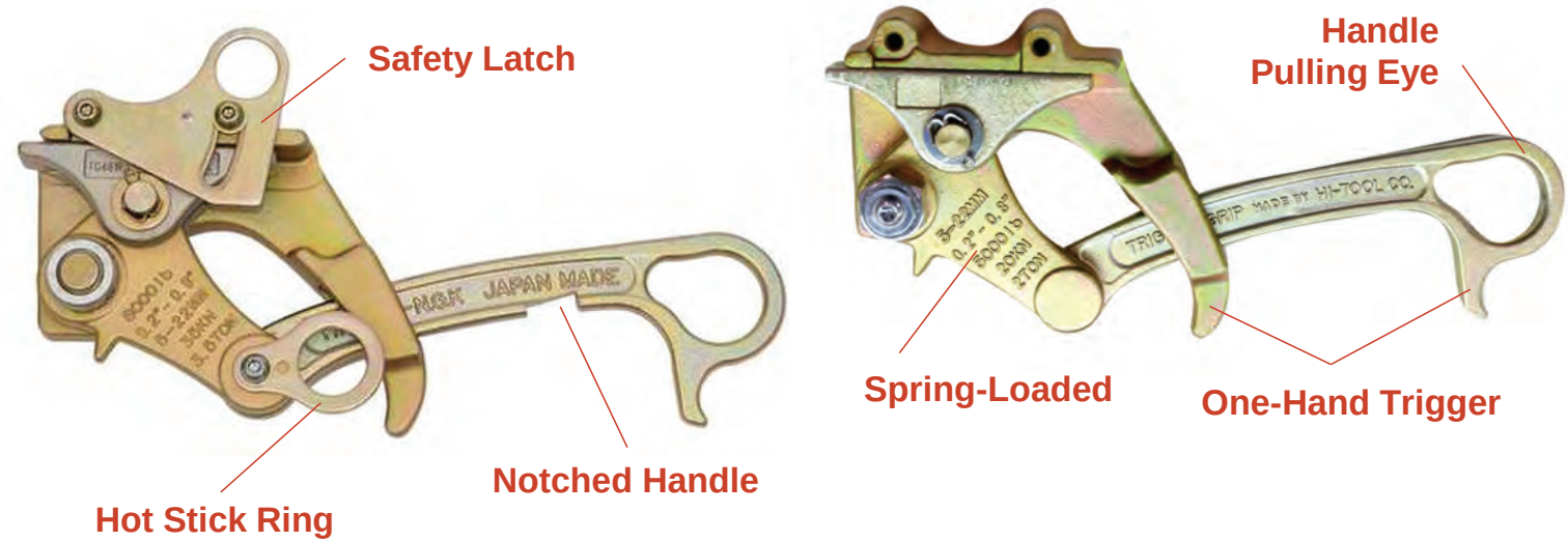
HOT LINE POWER GRIPS™ - with SPRING-LOADED SAFETY LATCH, HOT STICK RING, & NOTCHED HANDLE
