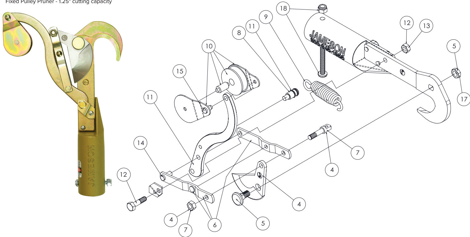
JA-14 Fixed Pulley Pruner - 1.25" cutting capacity
