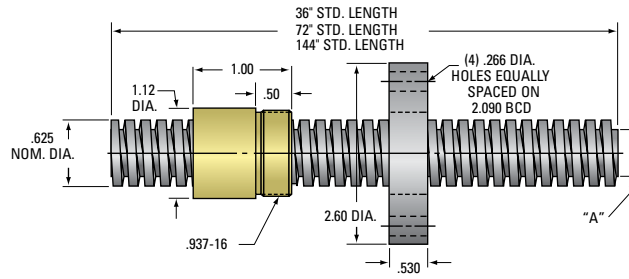
5/8" ACME THREAD Lead Accuracy 0.0003 in/in
