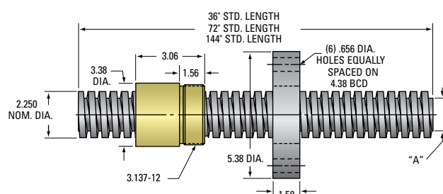
2 1/4" ACME THREAD Lead Accuracy 0.0003 in/in
