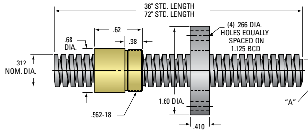
1/2" ACME THREAD Lead Accuracy 0.0003 in/in
