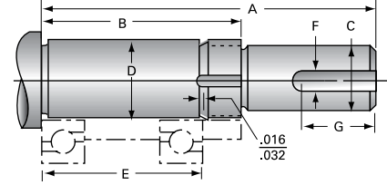
Type 3K (with keyway) Type 3L (without keyway)
