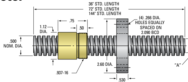
1/2" ACME THREAD Lead Accuracy 0.0003 in/in
