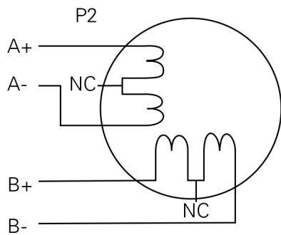
Figure 6: 6-lead motor full coil (higher torque) connections
