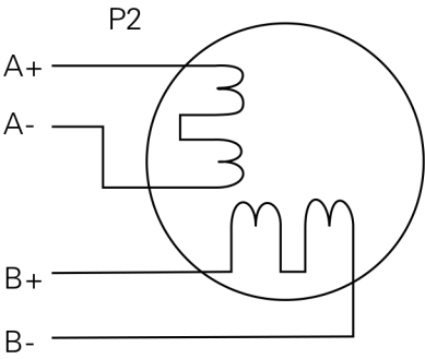
Figure 4: 4-lead Motor Connections
