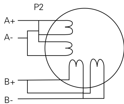
Figure 8: 8-lead motor parallel connections
