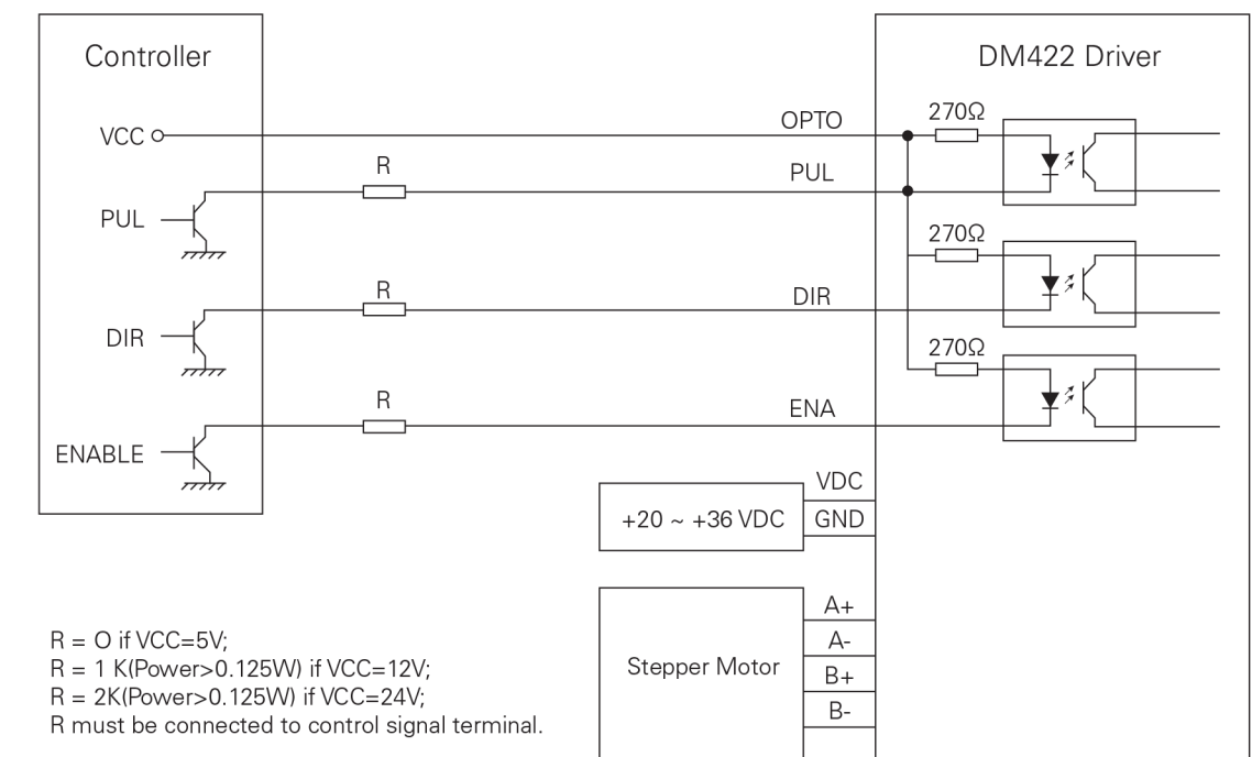
Figure 9: Typical connection
