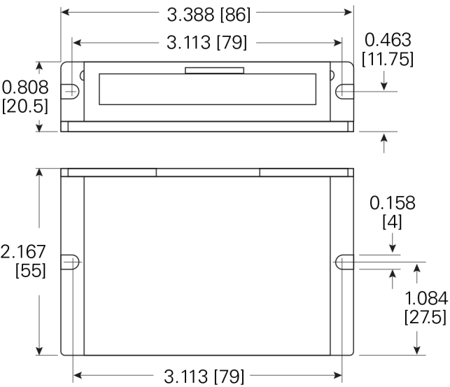
Mechanical Specifications ( unit: inch [mm] )
