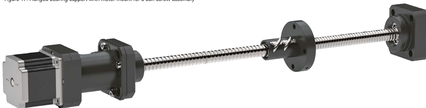
Figure 17: Flanged bearing support with motor mount for a ball screw assembly
