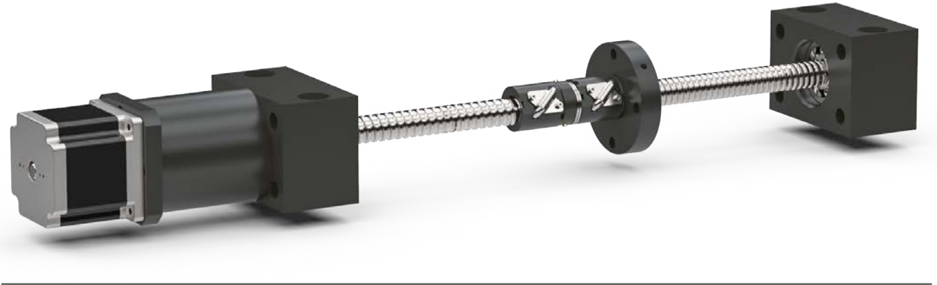
Figure 15: Universal bearing support with motor mount for a ball screw assembly
