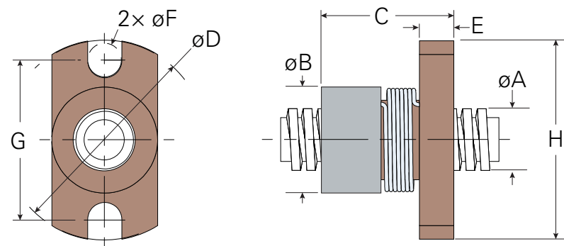
Rectangular Flange
