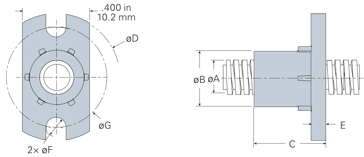
Two-Hole Flange Diameter Ranges: .078 – .188 in 2.0 – 5.0 mm
