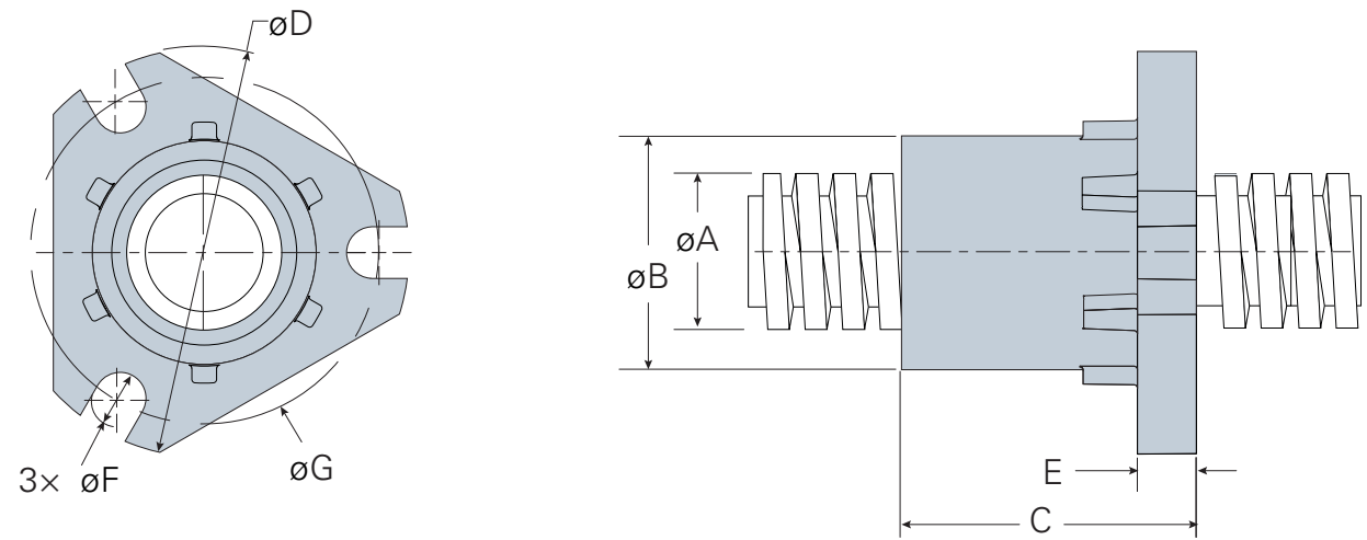
Three-Hole Flange Diameter Ranges: .195 – 1.000 in 5.5 – 25.4 mm
