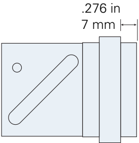
ø12.7 mm side view
