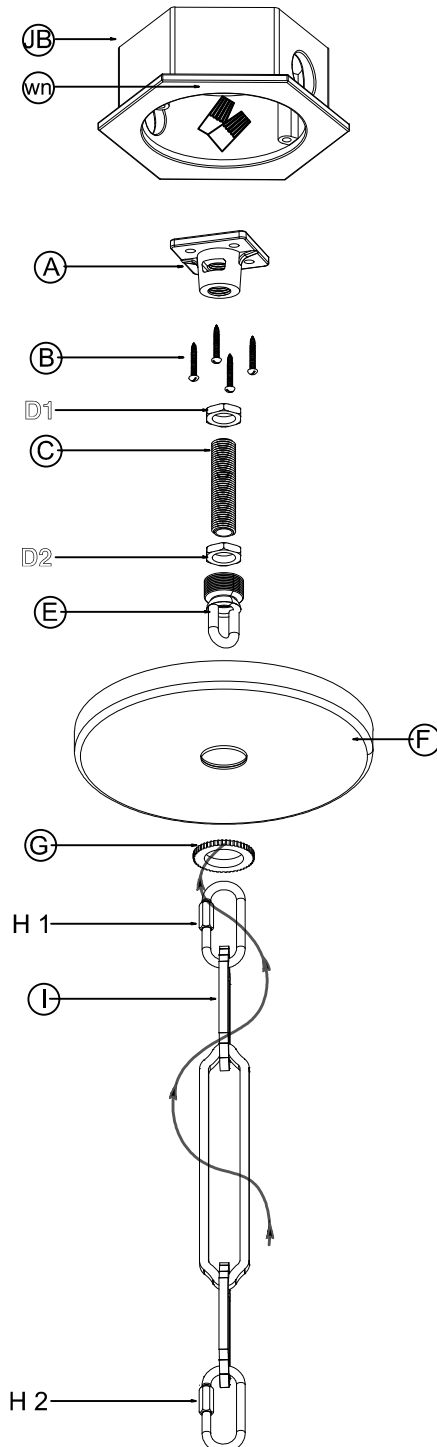
Drawing 2 – Canopy Adjustment
