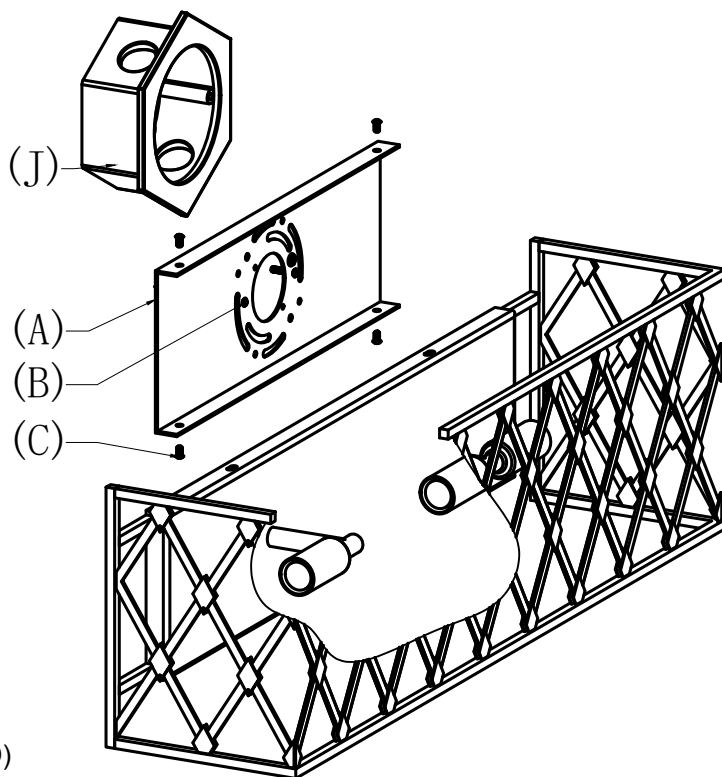
DRAWING-2
