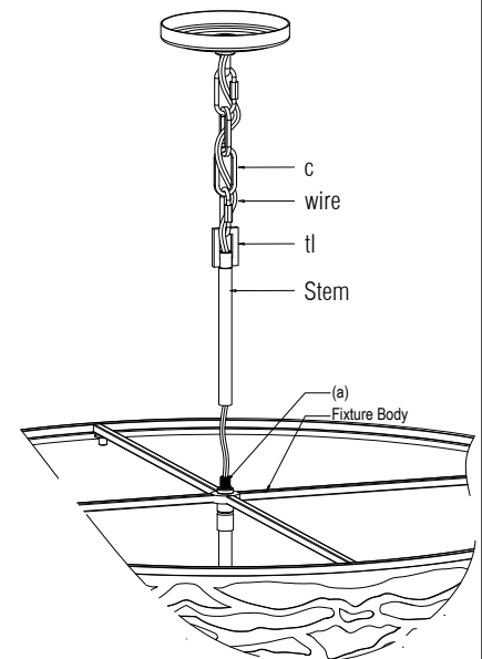
DRAWING-01
