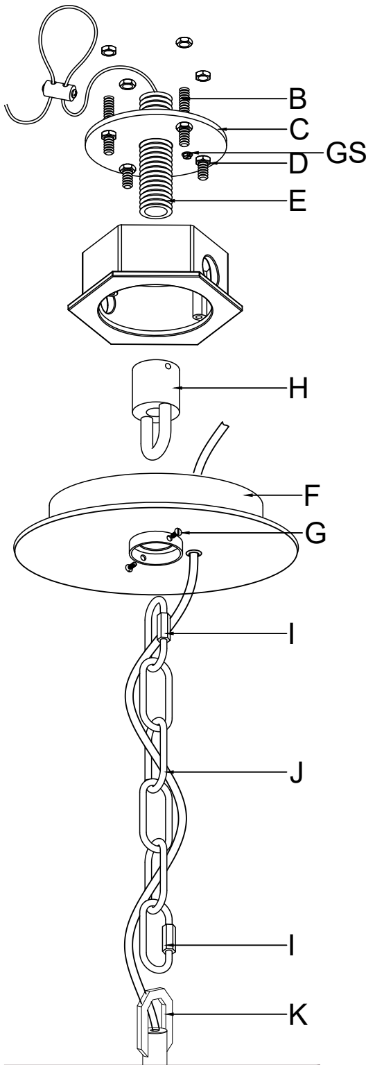
Drawing 2 – Canopy Adjustment
