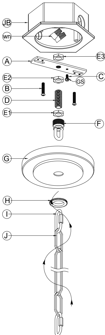
Drawing 1 – Hanging Instruction
