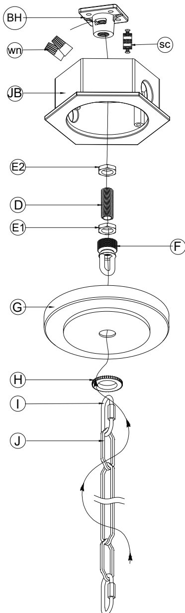
Drawing 1 – Hanging Instruction
