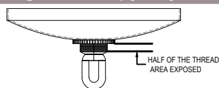
Drawing 2 – Canopy Adjustment
