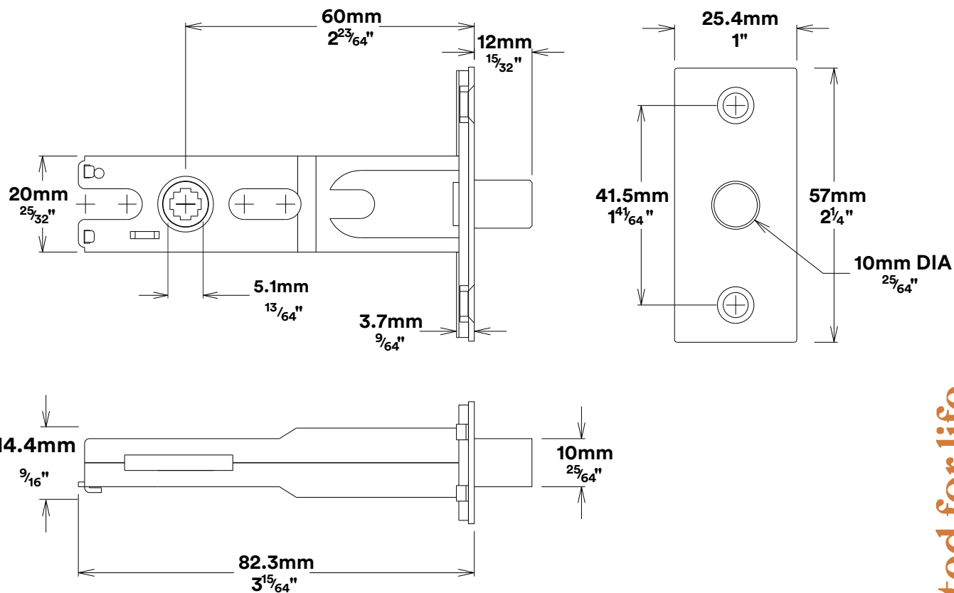
Privacy Bolt & Faceplate
