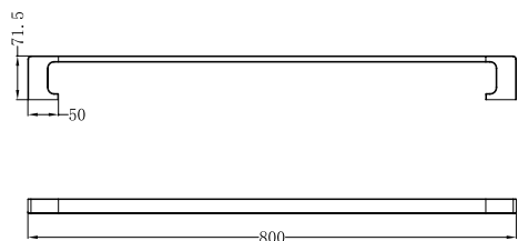
PEARL METAL SHOWER SHELF NR8087aCH/NR8087aMB/NR8087aGM
