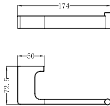
PEARL TOILET ROLL HOLDER NR8086CH/NR8086MB/NR8086GM
