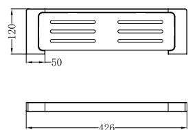
PEARL METAL SHOWER SHELF NR8087aCH/NR8087aMB/NR8087aGM
