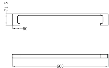
PEARL SINGLE TOWEL RAIL 600MM NR8024CH/NR8024MB/NR8024GM
