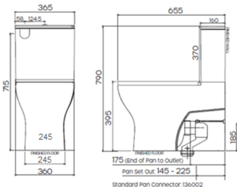
Optional Set Out Drawing
