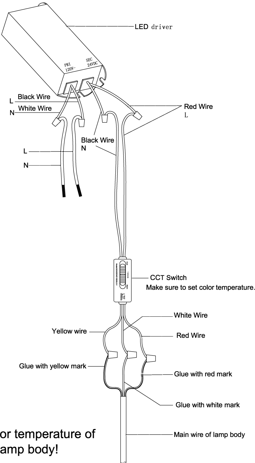
Wire connecting view
