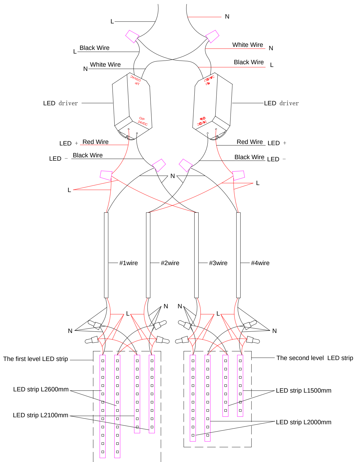
wire diagram
