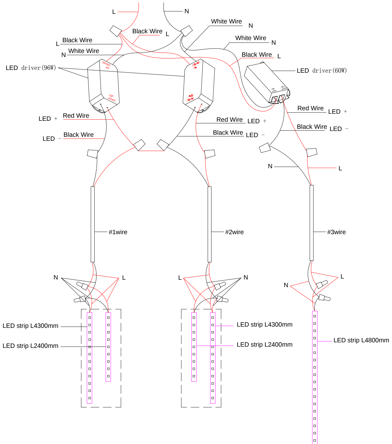
wire diagram
