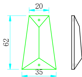
R20013-062-00-00 W35*W20*L62mm 156PCS
