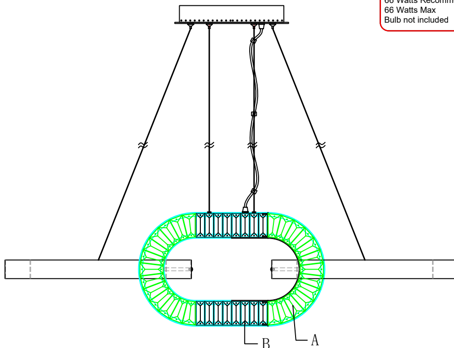
R20013-062-00-00 W35*W20*L62mm 156PCS
