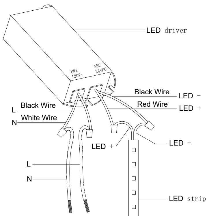
Wire connecting view
