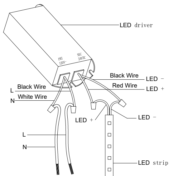
Wire connecting view
