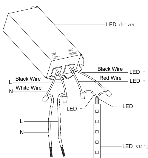
Wire connecting view
