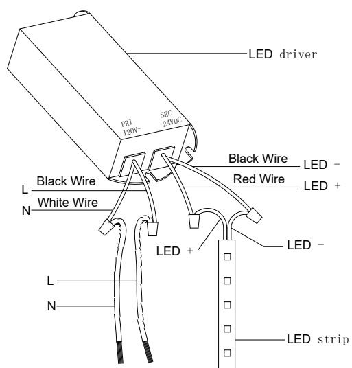
Wire connecting view
