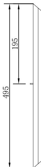
Hexagon clear crystal bar 20*L495mm R20006-495-00-01
