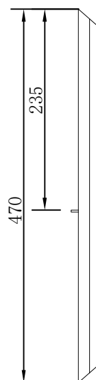
Hexagon clear crystal bar 20*L470mm R20006-470-00-00
