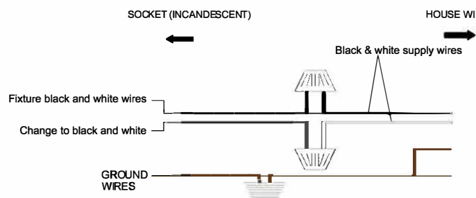
Wiring Diagram
