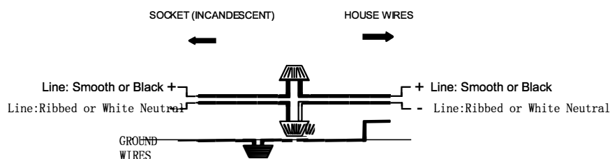
Wiring Diagram
