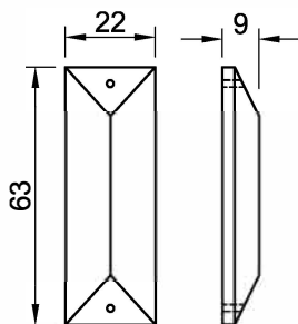
C R20610-063-00-01 W22*L63mm
