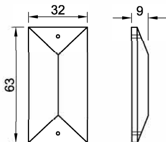
A Clear K9 crystal strip W32*L63*T9mm
