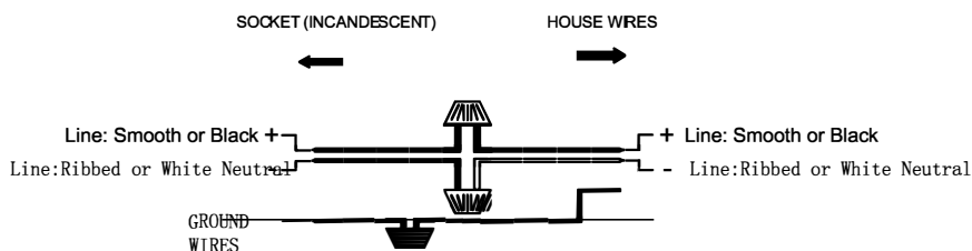
Wiring Diagram
