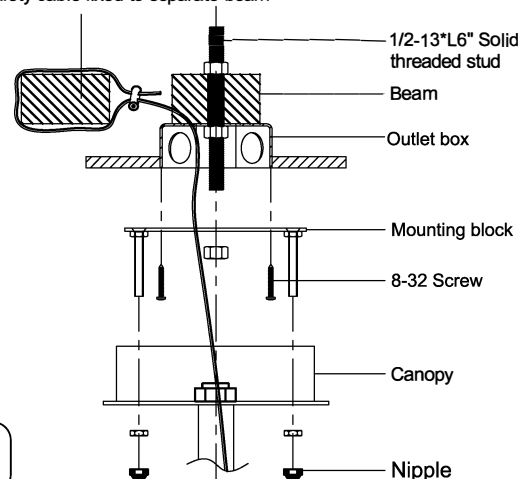
Safety cable fixed to separate beam
